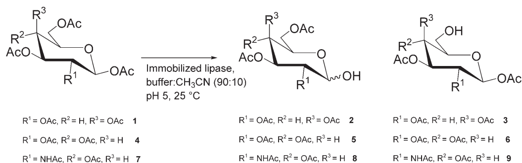
Scheme 1. Specific and regioselective hydrolysis of different 1,2,3,4,6-penta- O -acetyl- \beta -D-glycopyranoses.
