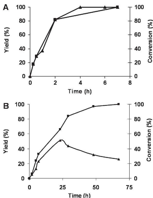
Figure 1. Reaction course of different immobilized preparations of TLL in the hydrolysis of 1 : A ) octyl-agarose preparation; B ) PEI-agarose preparation (squares = conversion, triangles = yield of monoprotected product).
